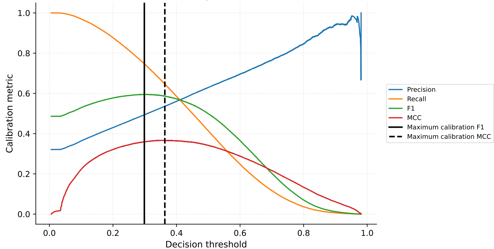
Calibration metric by decision threshold
