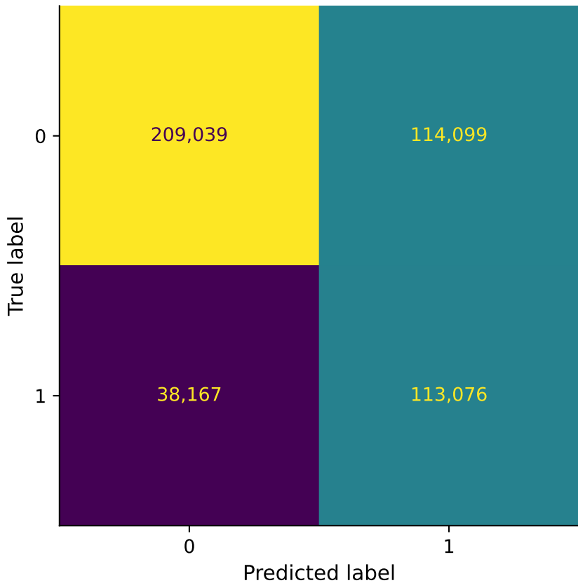
Test confusion matrix lightgbm_unweighted_optimized_average_precision
