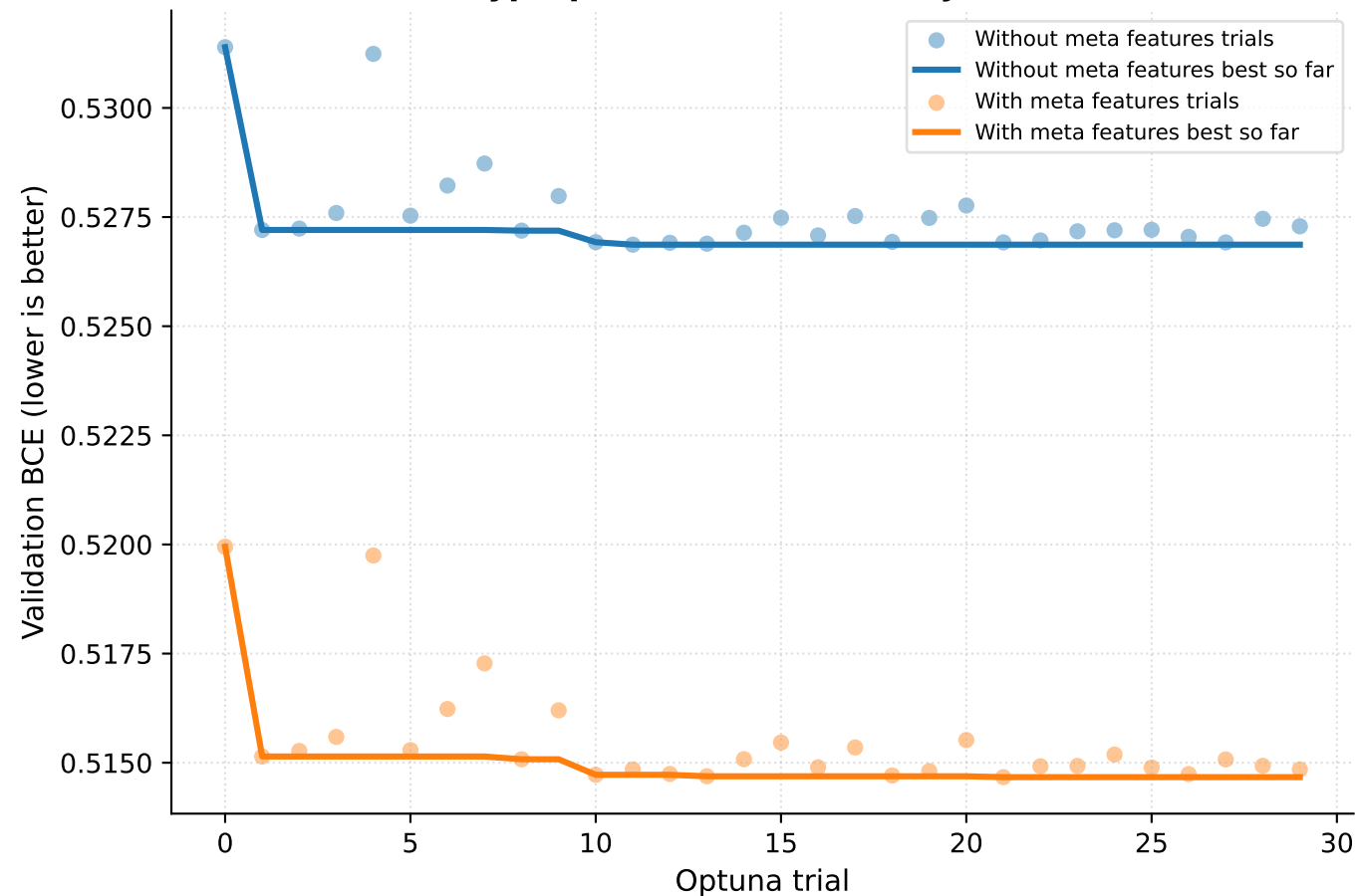
Hyperparameter search objective
