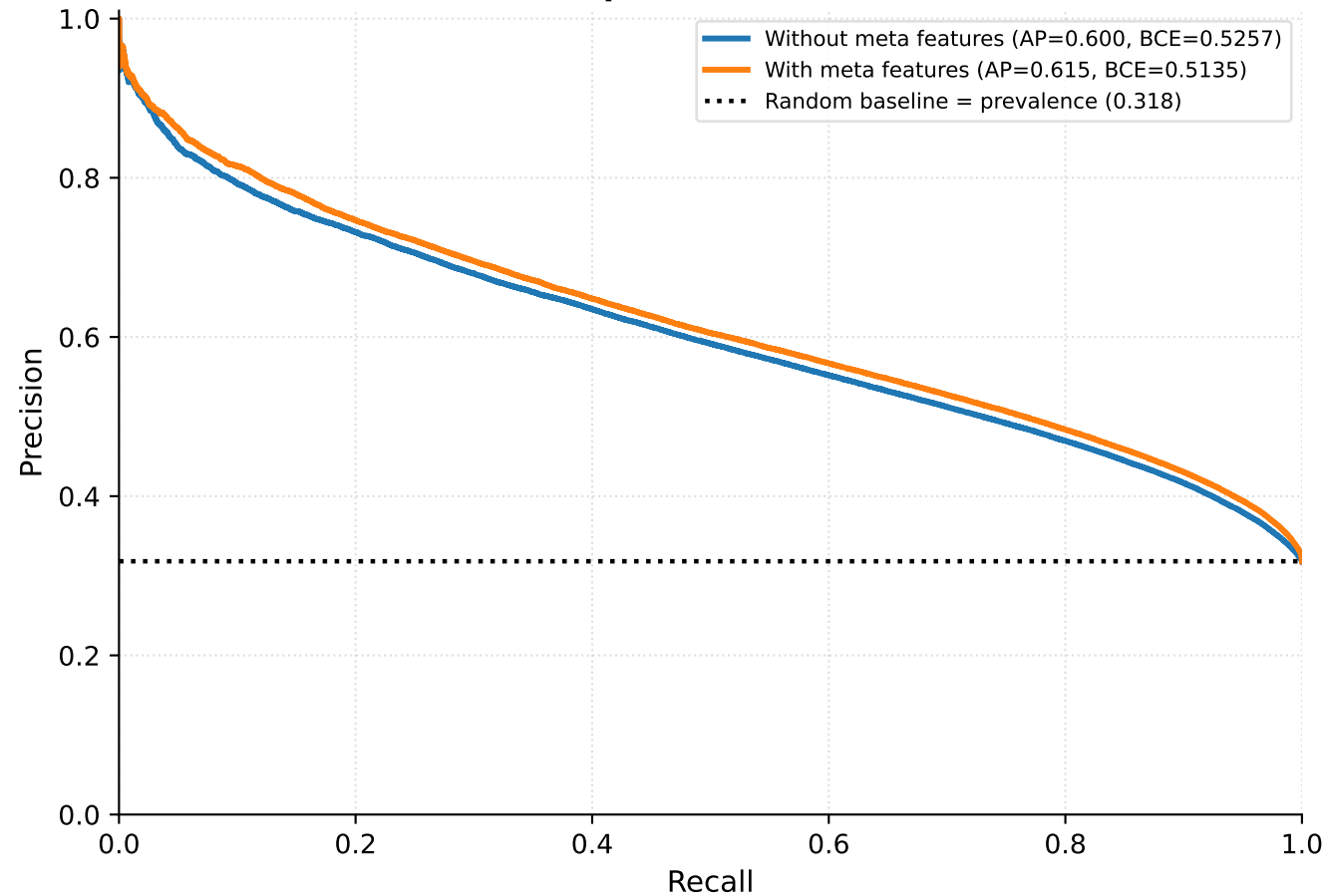
Validation precision-recall curves
