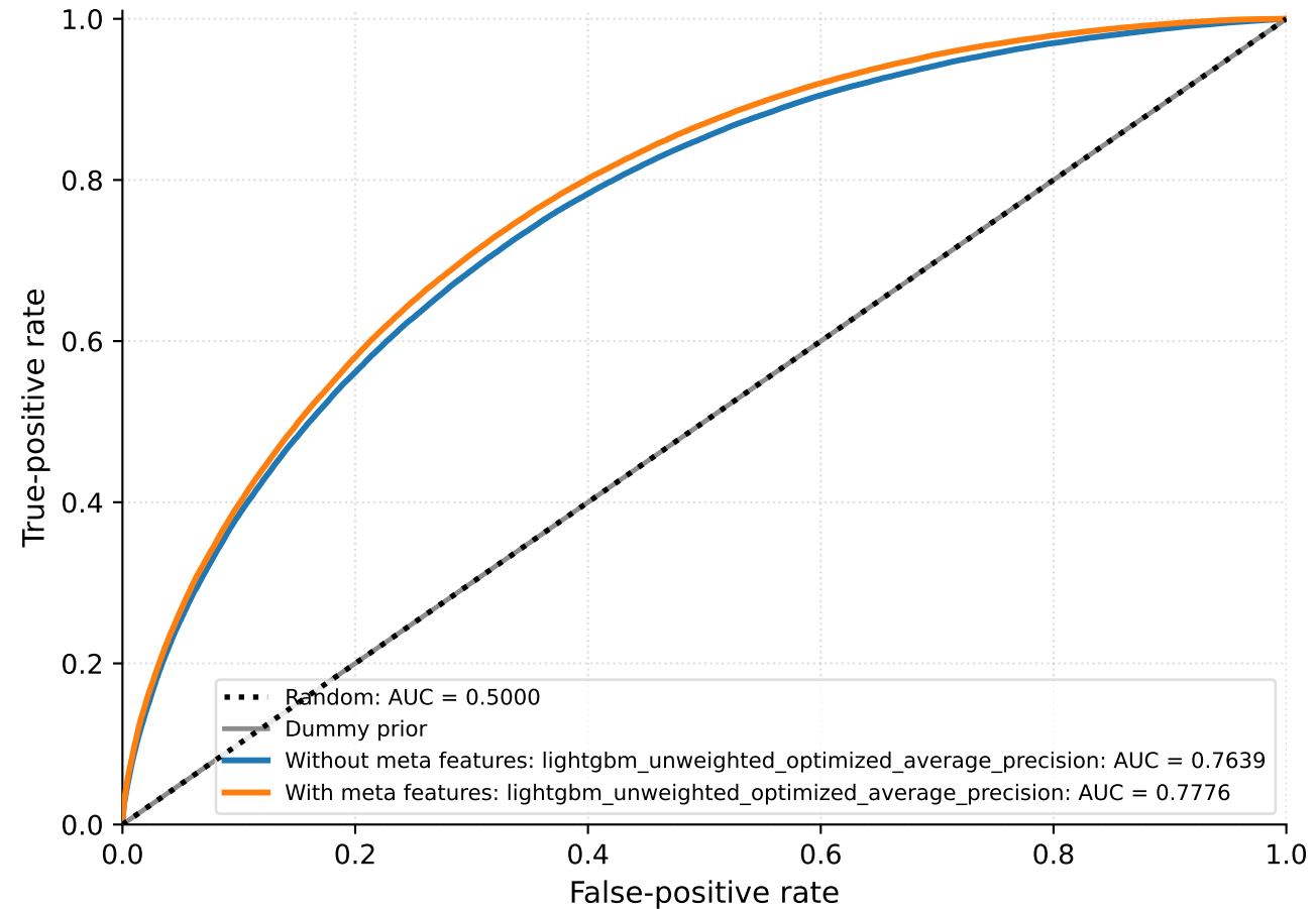
Validation ROC curves
