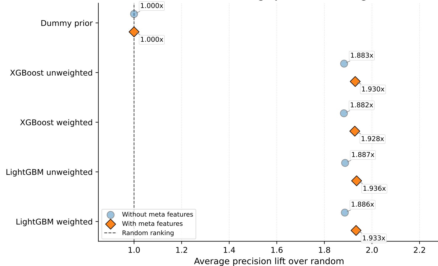
Validation average precision ranking
