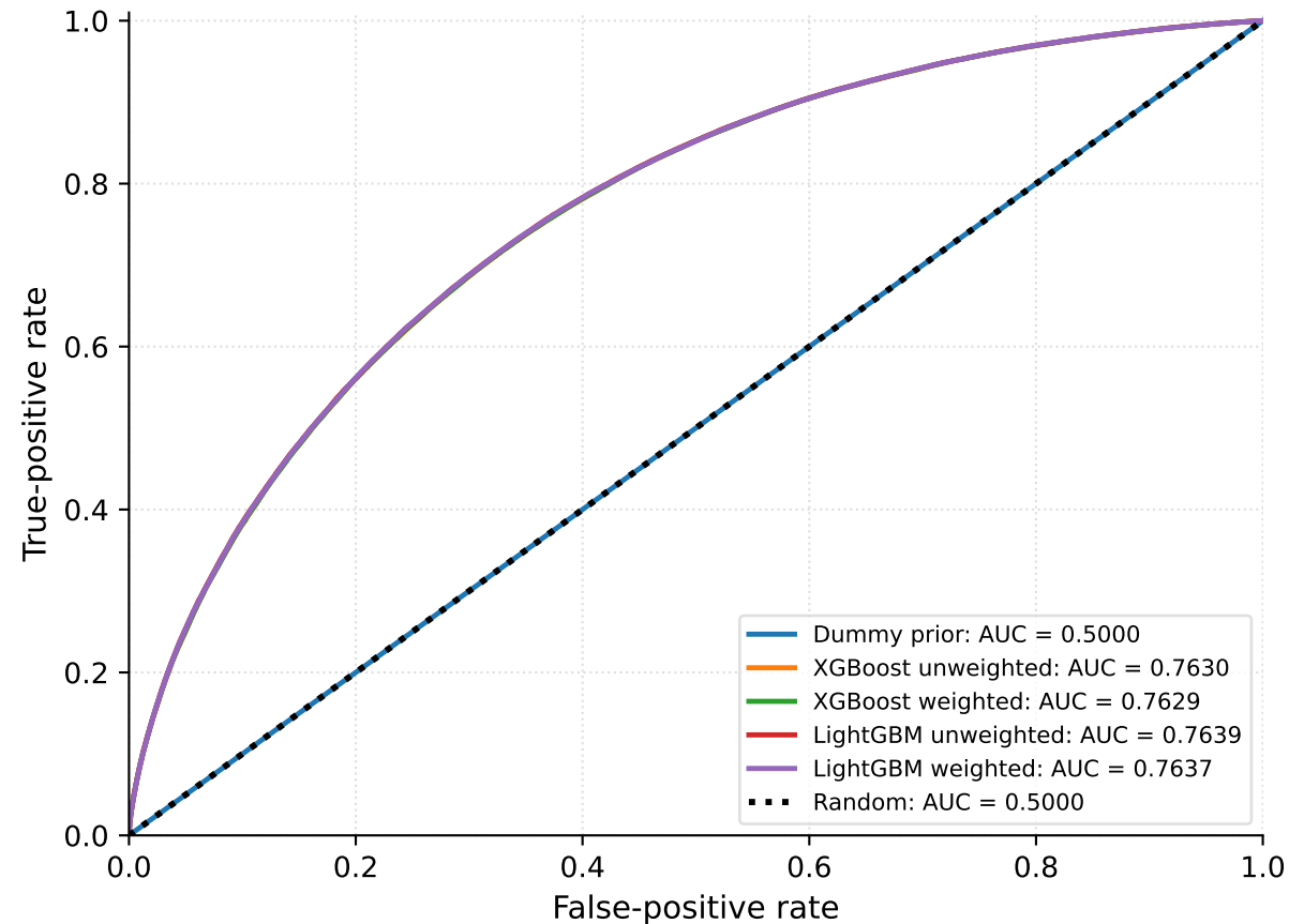
Validation ROC curves
