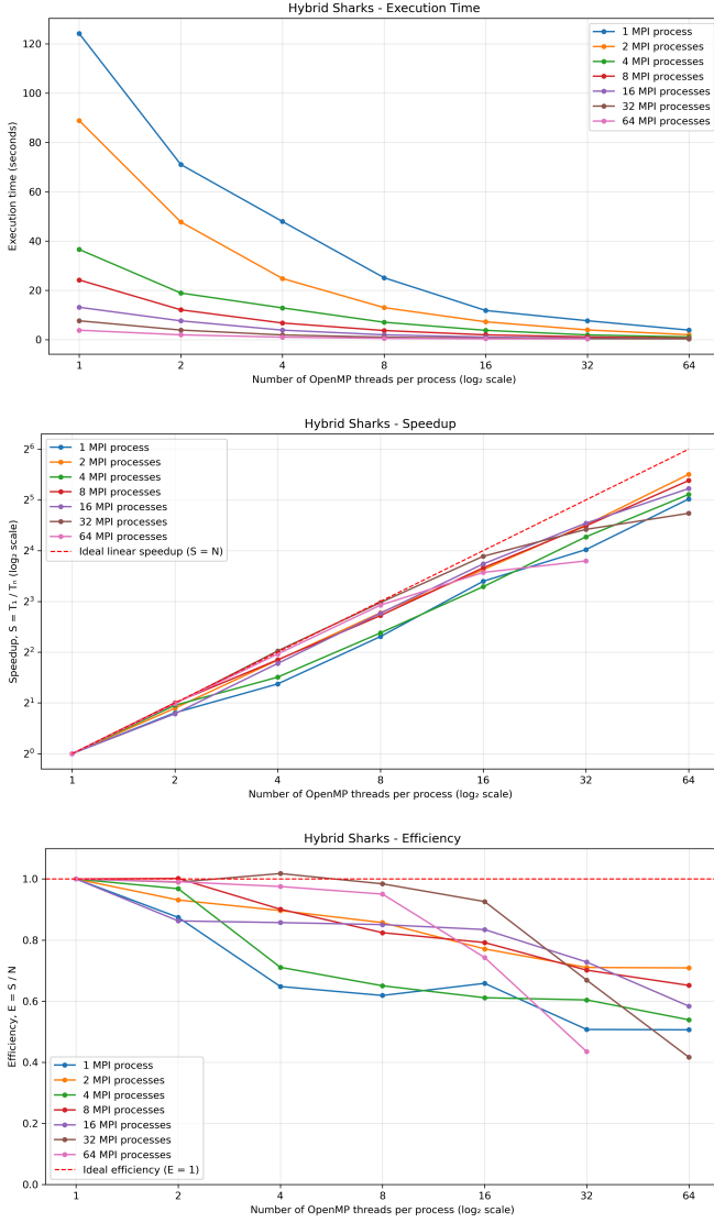
Fig. 7. Hybrid MPI+OpenMP shark-level implementation: execution time, speedup, and efficiency. Each line corresponds to a fixed number of MPI processes; the x-axis is the number of OpenMP threads per process.
