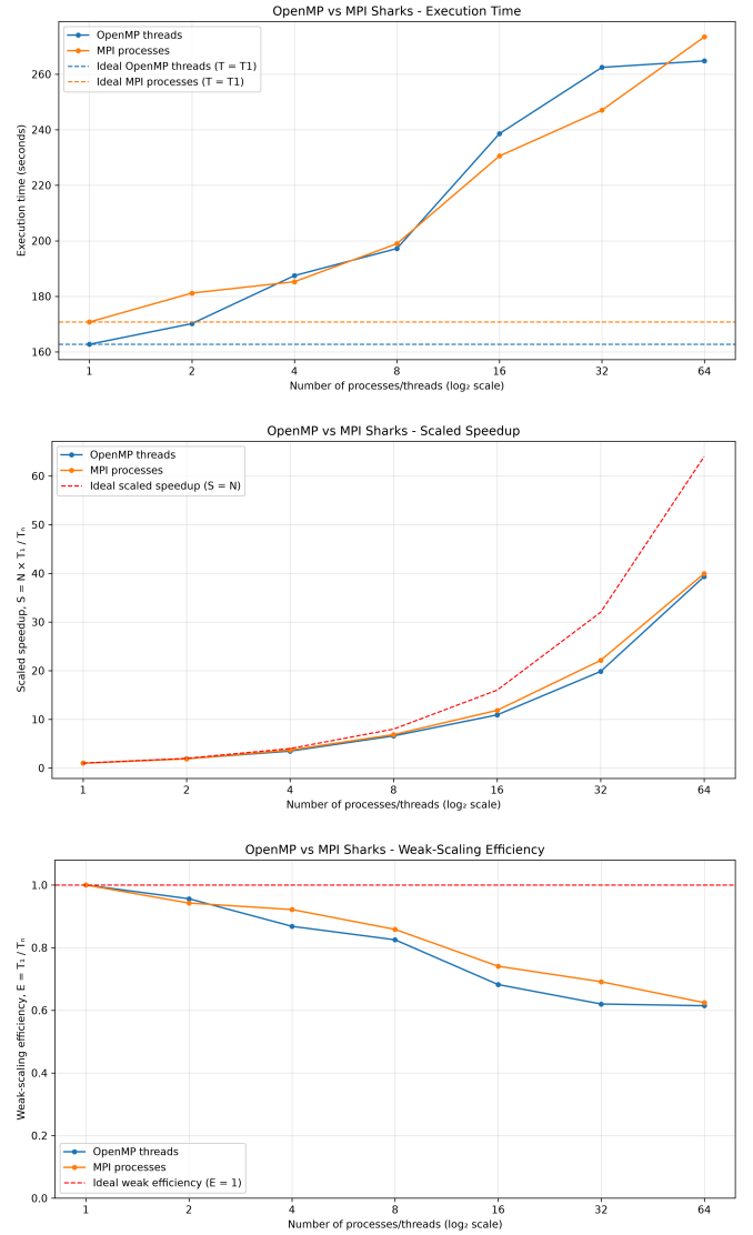
Fig. 13. Weak scaling, shark-level: execution time, speedup, and efficiency for MPI (processes) and OpenMP (threads) as the population grows with the worker count.
