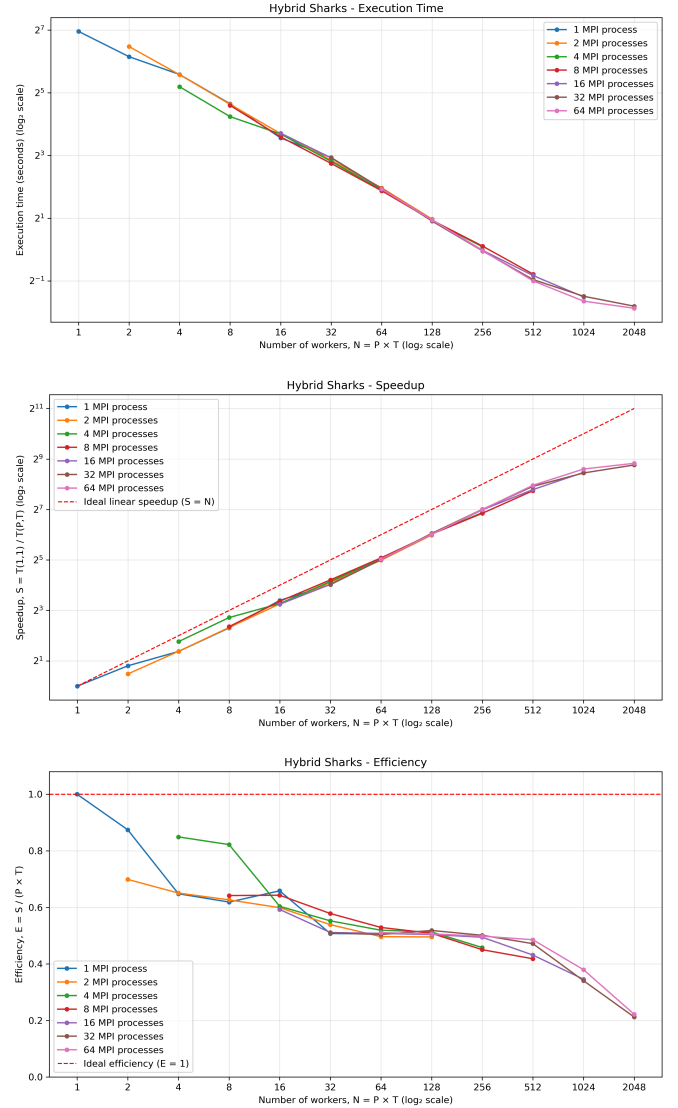
Fig. 8. Hybrid MPI+OpenMP shark-level implementation, global view: execution time, speedup, and efficiency measured against the serial baseline T(1,1) . Each line corresponds to a fixed number of MPI processes; the x-axis is the total number of workers P \times T on a log 2 scale.
