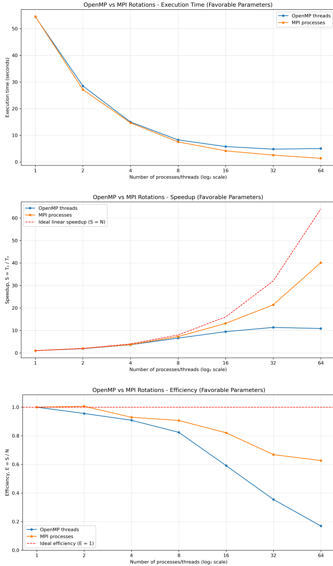
Fig. 12. Favorable rotation configuration ( M = 20000 ): execution time, speedup, and efficiency for MPI (processes) and OpenMP (threads).
