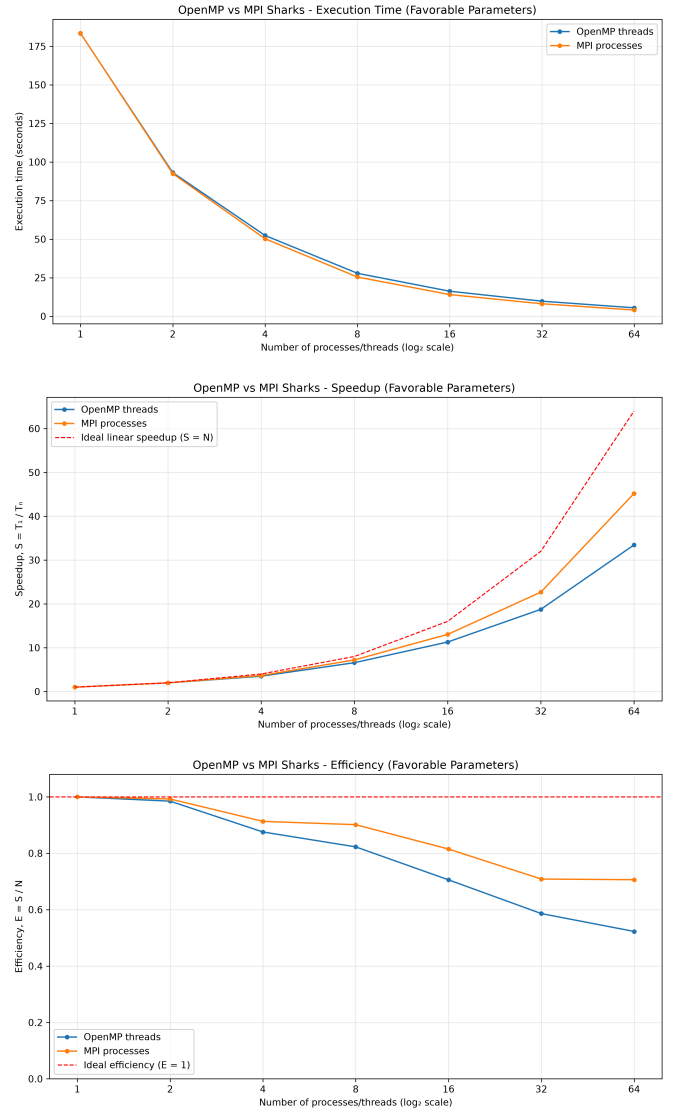
Fig. 9. Favorable shark configuration ( n_p = 8192 ): execution time, speedup, and efficiency for MPI (processes) and OpenMP (threads).
