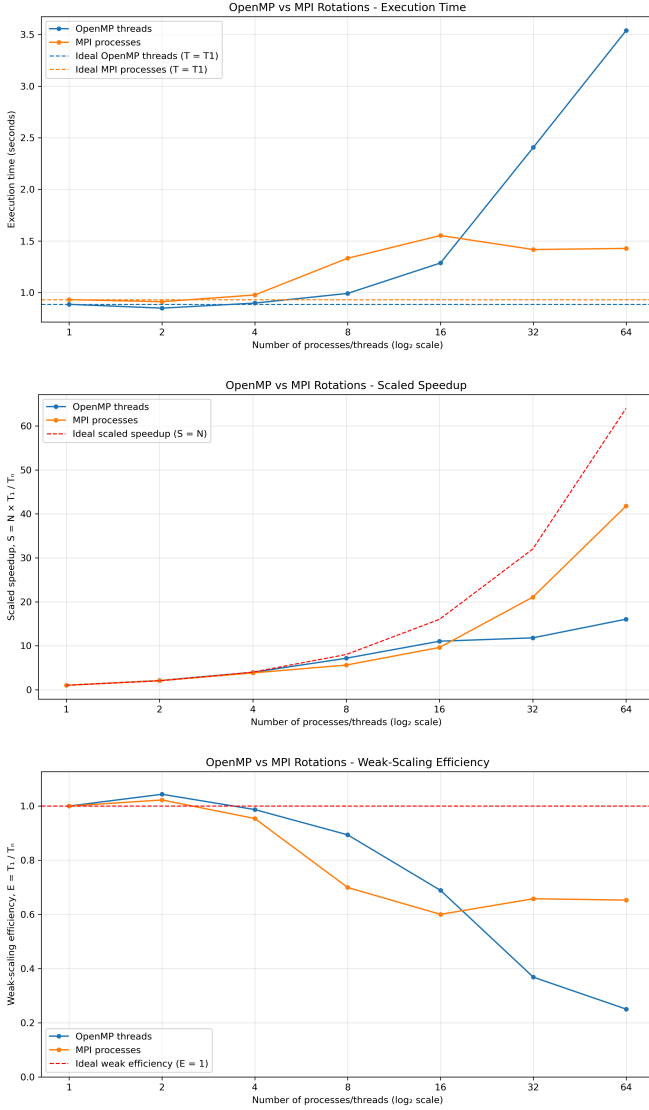
Fig. 16. Weak scaling, rotation-level: execution time, speedup, and efficiency for MPI (processes) and OpenMP (threads) as M grows with the worker count.
