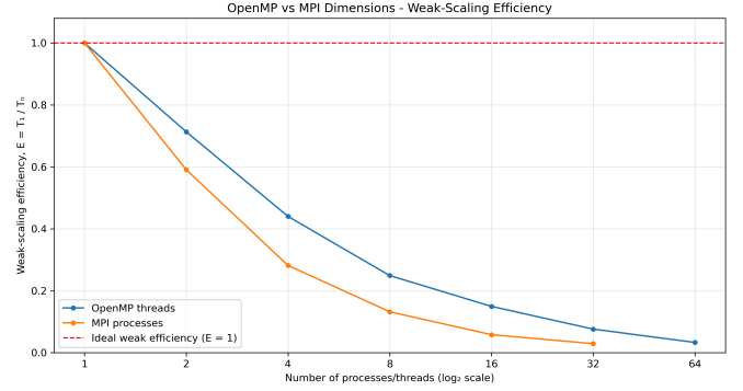
Fig. 15. Weak scaling, dimension-level: execution time, speedup, and efficiency for MPI (processes) and OpenMP (threads) as n_d grows with the worker count.
