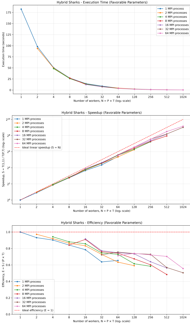
Fig. 10. Favorable shark configuration ( np = 8192 ), hybrid MPI+OpenMP: execution time, speedup, and efficiency against the serial baseline.
