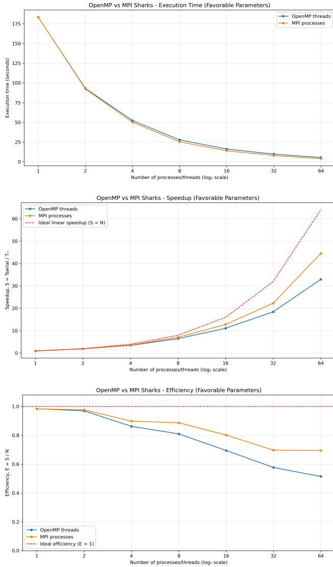
Fig. 8. Favorable shark configuration ( n_p = 8192 ): execution time, speedup, and efficiency for MPI (processes) and OpenMP (threads).
