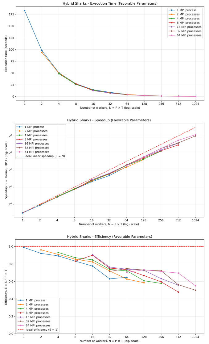
Fig. 9. Favorable shark configuration ( n_p = 8192 ), hybrid MPI+OpenMP: execution time, speedup, and efficiency against the serial baseline.
