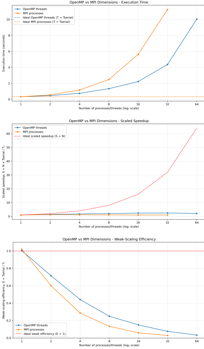
Fig. 14. Weak scaling, dimension-level: execution time, speedup, and efficiency for MPI (processes) and OpenMP (threads) as nd grows with the worker count.
