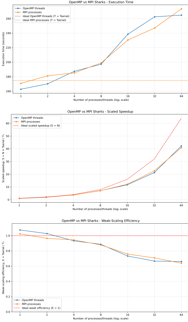
Fig. 12. Weak scaling, shark-level: execution time, speedup, and efficiency for MPI (processes) and OpenMP (threads) as the population grows with the worker count.
