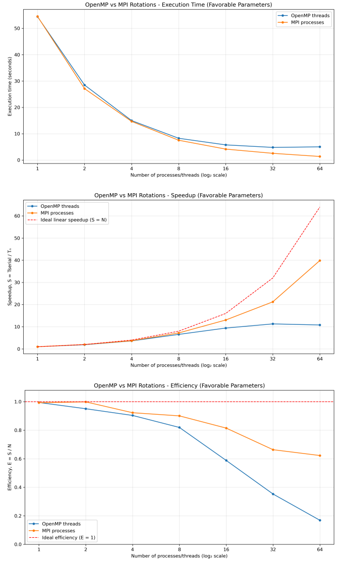
Fig. 11. Favorable rotation configuration ( M = 20000 ): execution time, speedup, and efficiency for MPI (processes) and OpenMP (threads).
