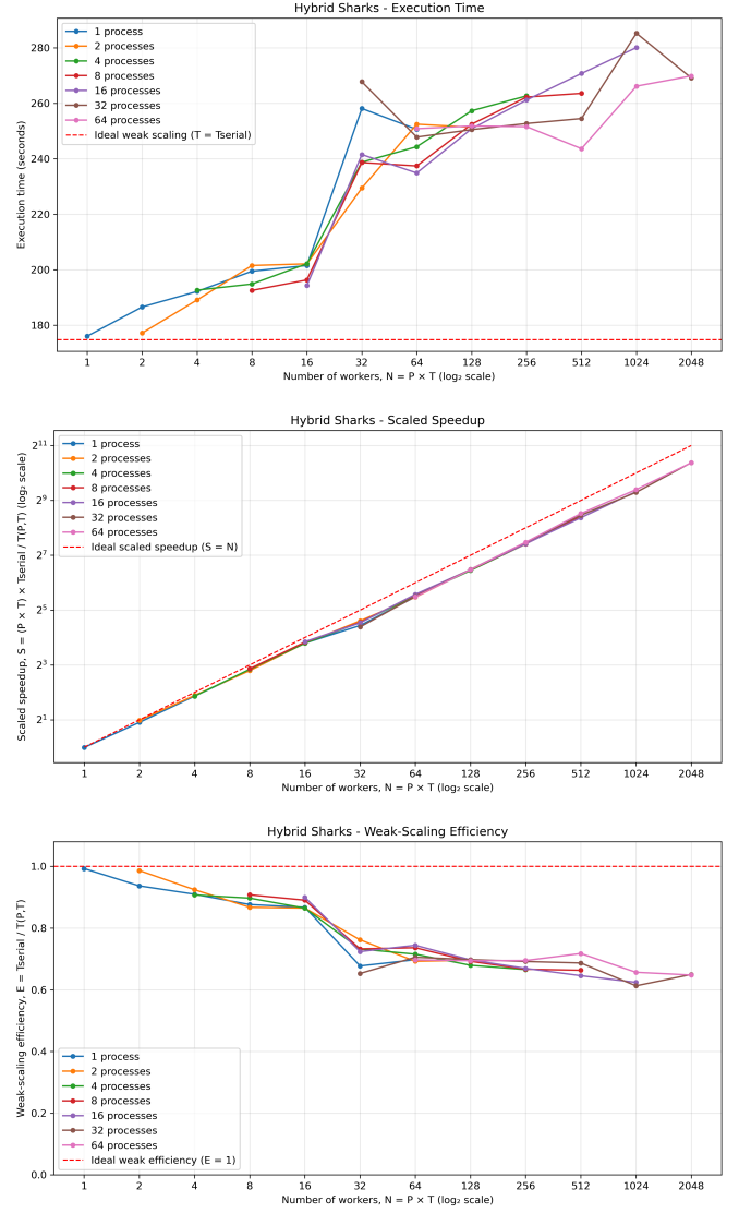
Fig. 13. Weak scaling, hybrid MPI+OpenMP shark-level: execution time, speedup, and efficiency as the population grows with the worker count.
