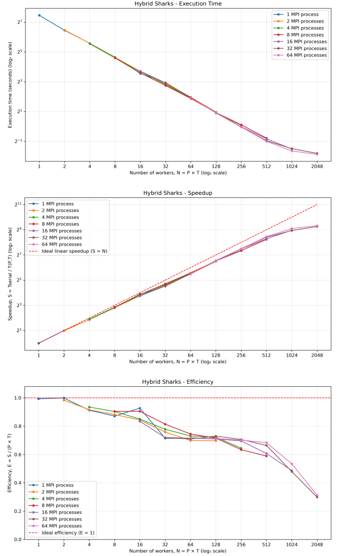
Fig. 7. Hybrid MPI+OpenMP shark-level implementation, global view: execution time, speedup, and efficiency measured against the serial baseline T(1,1) . Each line corresponds to a fixed number of MPI processes; the x-axis is the total number of workers P \times T on a log 2 scale.
