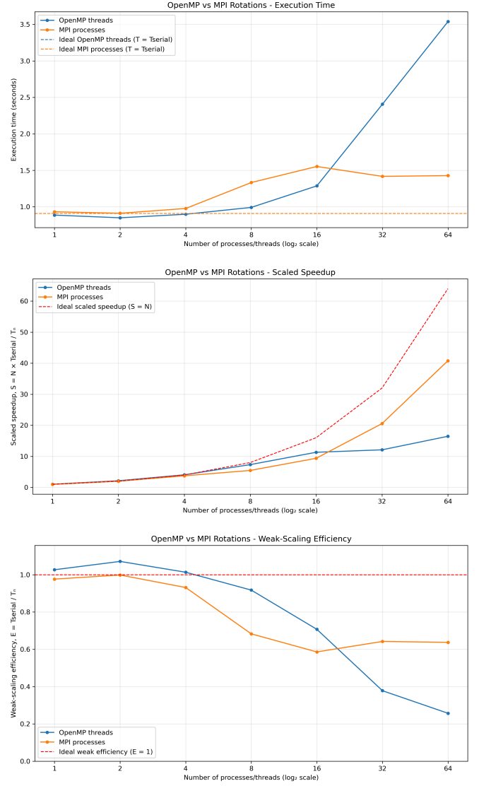
Fig. 15. Weak scaling, rotation-level: execution time, speedup, and efficiency for MPI (processes) and OpenMP (threads) as M grows with the worker count.
