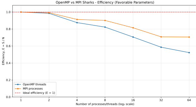
Fig. 9. Favorable shark configuration ( np = 8192 ): execution time, speedup, and efficiency for MPI (processes) and OpenMP (threads).
