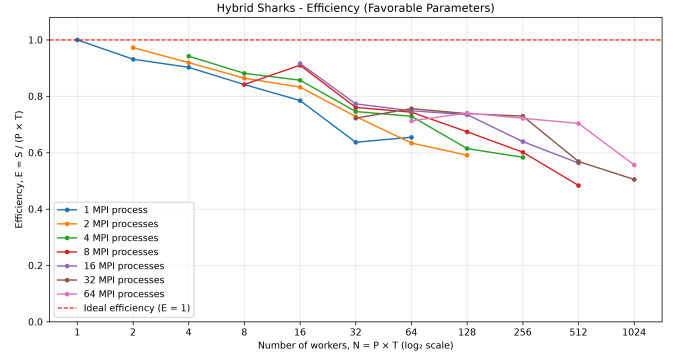
Fig. 10. Favorable shark configuration ( np = 8192 ), hybrid MPI+OpenMP: execution time, speedup, and efficiency against the serial baseline.
