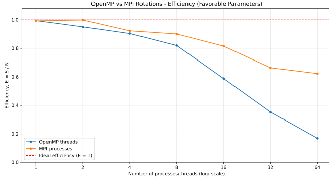
Fig. 11. Favorable rotation configuration ( M = 20000 ): execution time, speedup, and efficiency for MPI (processes) and OpenMP (threads).
