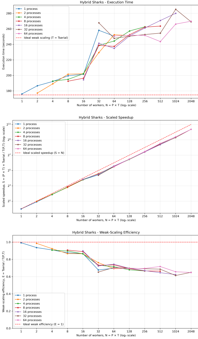
Fig. 13. Weak scaling, hybrid MPI+OpenMP shark-level: execution time, speedup, and efficiency as the population grows with the worker count.
