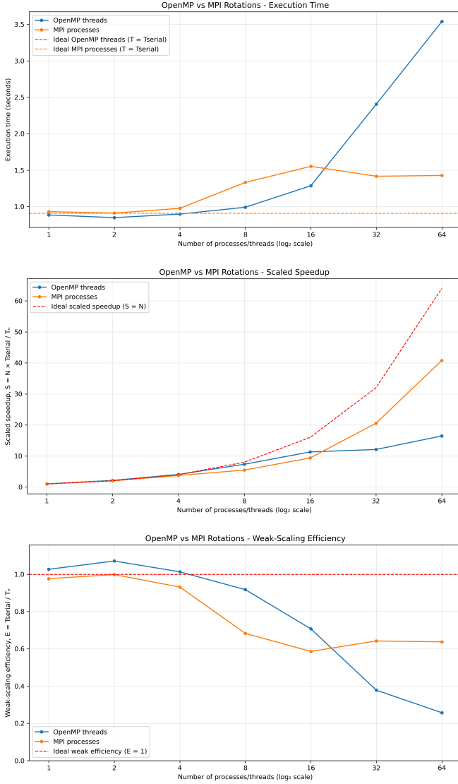
Fig. 15. Weak scaling, rotation-level: execution time, speedup, and efficiency for MPI (processes) and OpenMP (threads) as M grows with the worker count.
