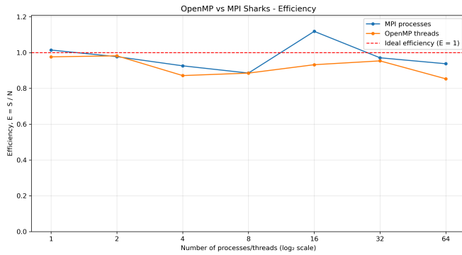
Fig. 4. Shark-level decomposition: execution time, speedup, and efficiency for MPI (processes) and OpenMP (threads).
