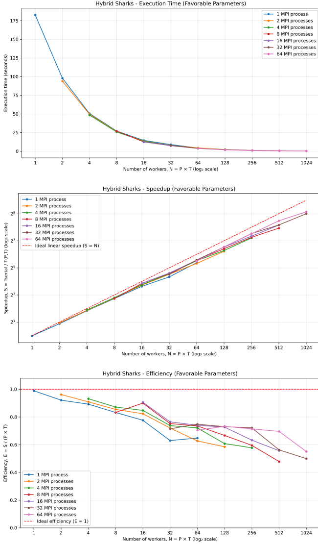
Fig. 9. Favorable shark configuration ( n_p = 8192 ), hybrid MPI+OpenMP: execution time, speedup, and efficiency against the serial baseline.
