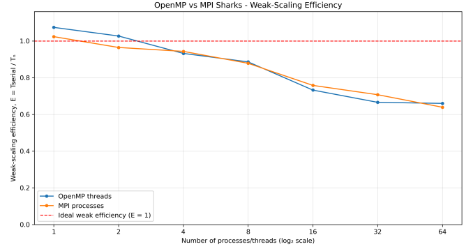
Fig. 12. Weak scaling, shark-level: execution time, speedup, and efficiency for MPI (processes) and OpenMP (threads) as the population grows with the worker count.
