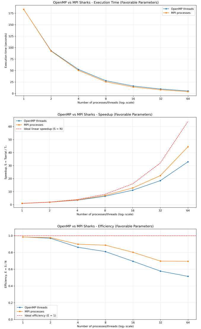
Fig. 8. Favorable shark configuration ( n_p = 8192 ): execution time, speedup, and efficiency for MPI (processes) and OpenMP (threads).
