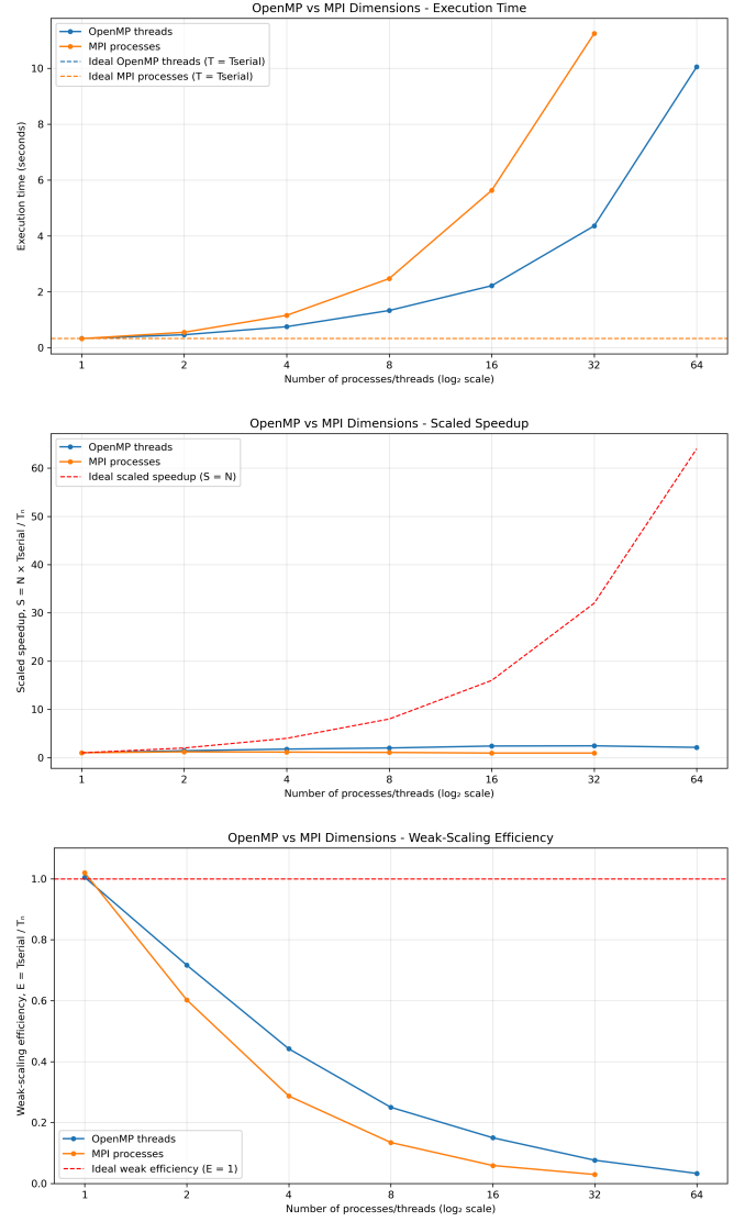
Fig. 14. Weak scaling, dimension-level: execution time, speedup, and efficiency for MPI (processes) and OpenMP (threads) as n_d grows with the worker count.
