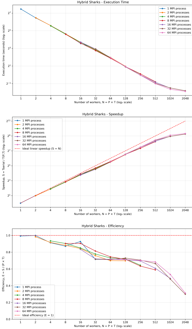
Fig. 7. Hybrid MPI+OpenMP shark-level implementation, global view: execution time, speedup, and efficiency measured against the serial baseline T_{\text{ser}} . Each line corresponds to a fixed number of MPI processes; the x-axis is the total number of workers P \times T on a log 2 scale.
