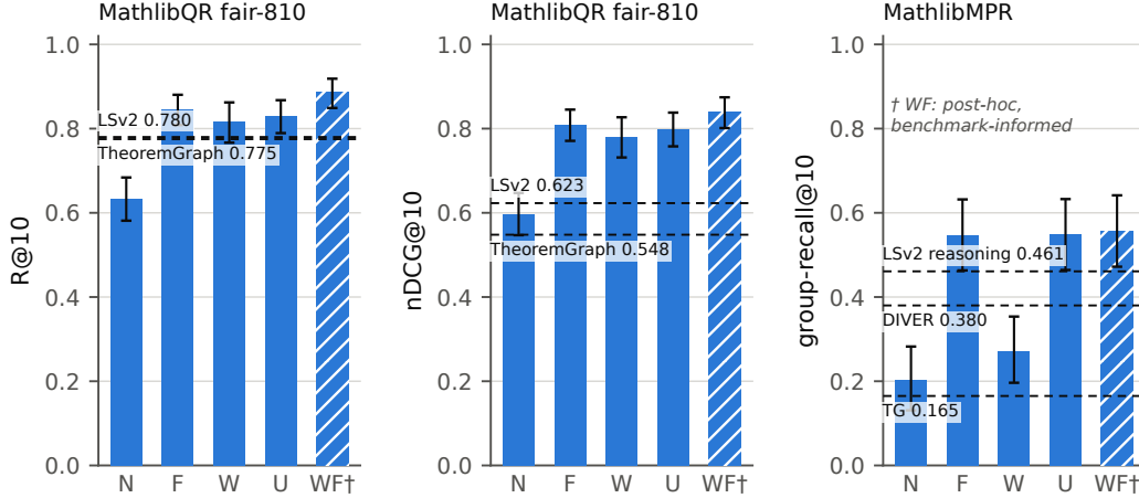
Figure 2: The repaired-grid five-arm retrieval results (exploratory) with declaration-clustered (QR) and task-bootstrap (MPR) 95% confidence whiskers (the exact asymmetric bounds), against the published anchors (dashed). Arms: N = no tools; F = formal search; W = the Brain; U = the bare W \cup F union, no manual; WF = union + manual. WF (hatched) is post-hoc and benchmark-informed (§5, Supplement §S8); published anchors are single-call systems (MPR: LSv2’s reasoning mode is itself iterative) — context, not controlled comparison. Source: grid_repaired.json , union_ablation.json .
