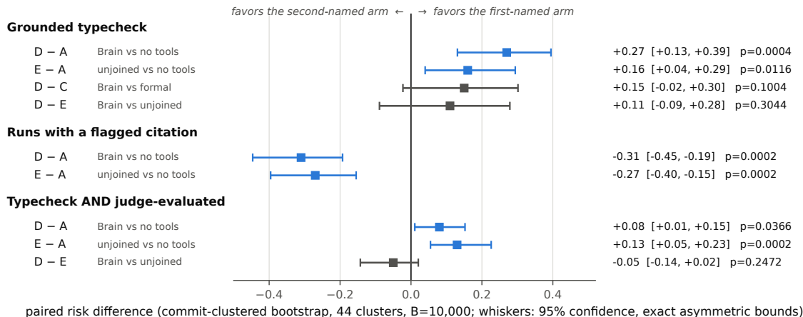
Figure 1: Headline contrasts of the fresh-100 study, grouped by outcome (repaired instrument). Arms: A = no tools; C = formal search; D = the Brain (join + verifier); E = both corpora, unjoined. Rows: each row is a paired comparison — e.g. D - A is the Brain arm’s rate minus the no-tools arm’s rate on the same 100 tasks, in percentage points (plotted as proportions: +0.27 = +27 points). Reading: points right of zero favor the first-named arm; whiskers are 95% confidence (commit-clustered bootstrap, 44 clusters, B=10,000 — the exact asymmetric bounds behind the \pm values in the text); a whisker crossing zero means the comparison is inconclusive; blue intervals exclude zero. Outcome groups: grounded typecheck (§4.1); runs with a flagged (hallucinated) citation (§4.3 — RDs are negative because fewer flags are better, and flagged rates are upper bounds on true hallucination, §4.1); and the grounded-typecheck \wedge judged-equivalent conjunction (§4.2). Register: the first two groups are corrective-exploratory (the preregistered endpoint was never graded, §3.3); the conjunction adds the uncalibrated-judge leg and is exploratory only. Sources: success_repaired.json , v3_gate_fixes.json .
