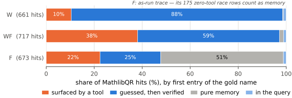
Figure 3: Provenance decomposition of MathlibQR hits (exploratory): where the gold name first entered the transcript. Arms as in Figure 2 (W = the Brain, WF = union + manual, F = formal search). “Guessed, then verified” means the model wrote the name and decl_exists (or another tool) confirmed it; the residual sliver is names present in the query itself. The trace pass is as-run — F’s 175 zero-tool race rows count as memory, an upper bound (§5). Source: retrieval_provenance.json .
