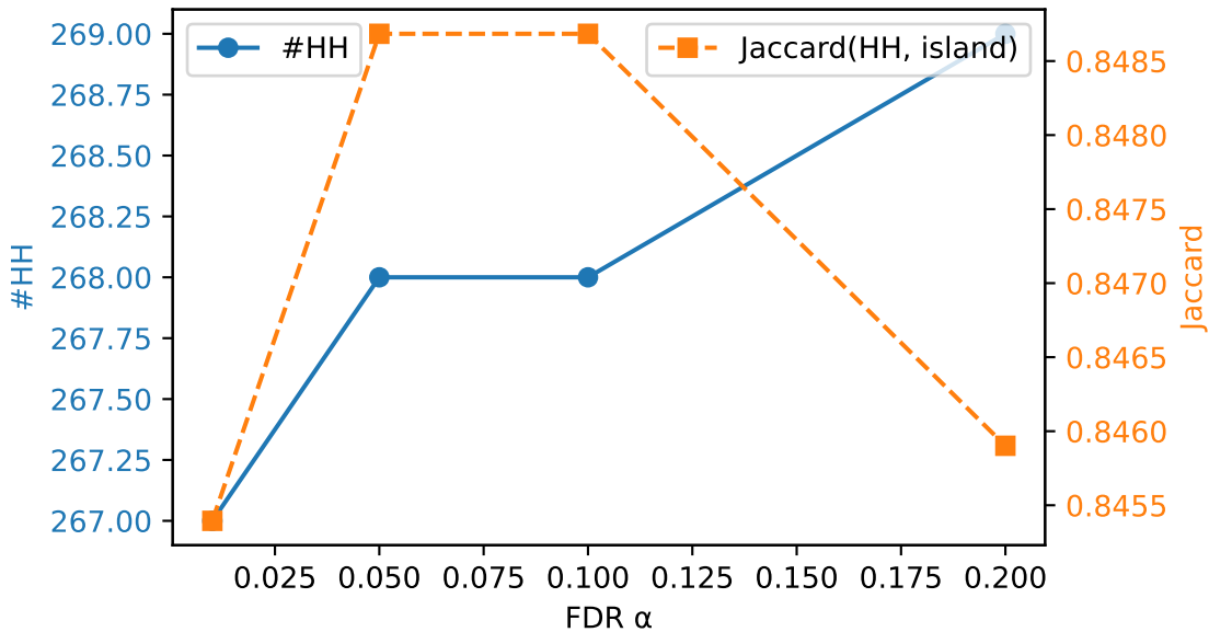
FDR \alpha sensitivity (three islands)
