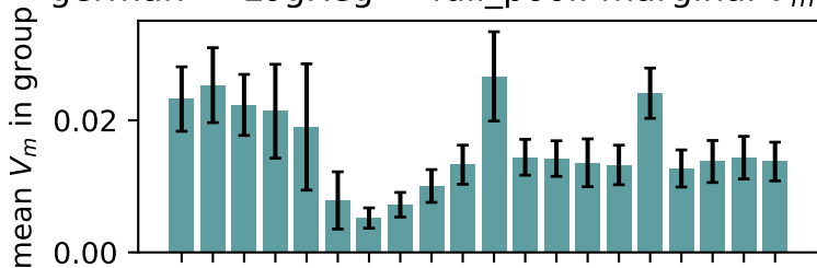
german — LogReg — full_pool: marginal V_m by C
