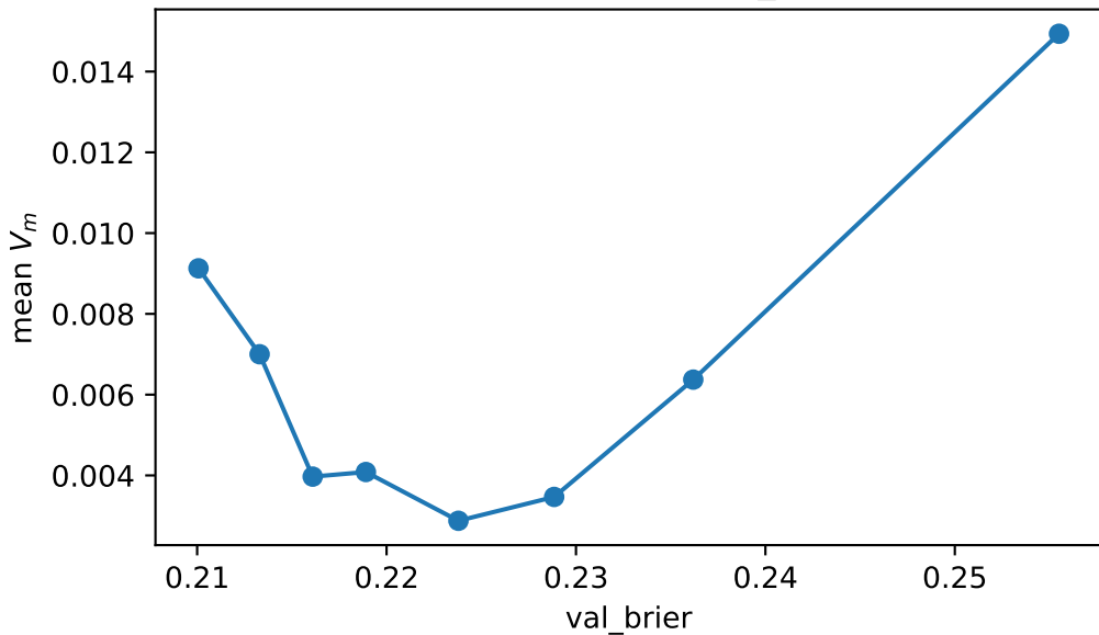
compas — RF — full_pool
