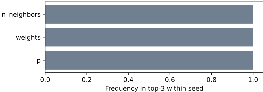
adult — kNN: rank stability (V_m importance, subset=all)
