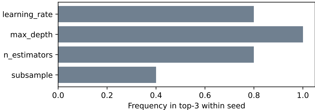
compas — GBM: rank stability (V_m importance, subset=all)
