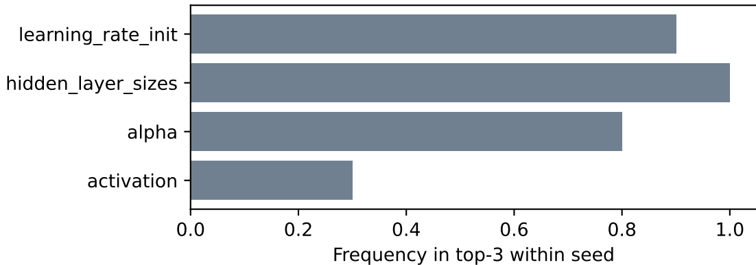
compas — MLP: rank stability (V_m importance, subset=all)
