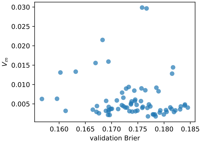
german — kNN — Rashomon
