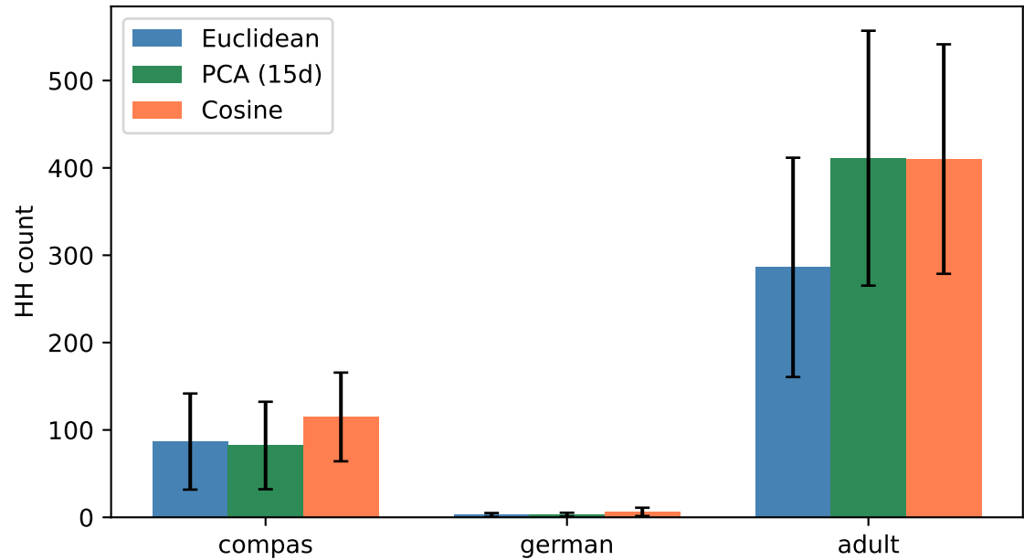
HH count
