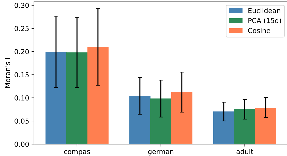
Moran's I
