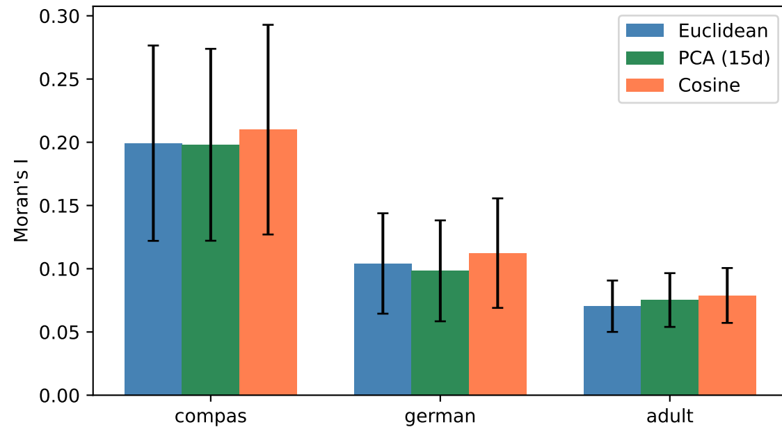
Moran's I
