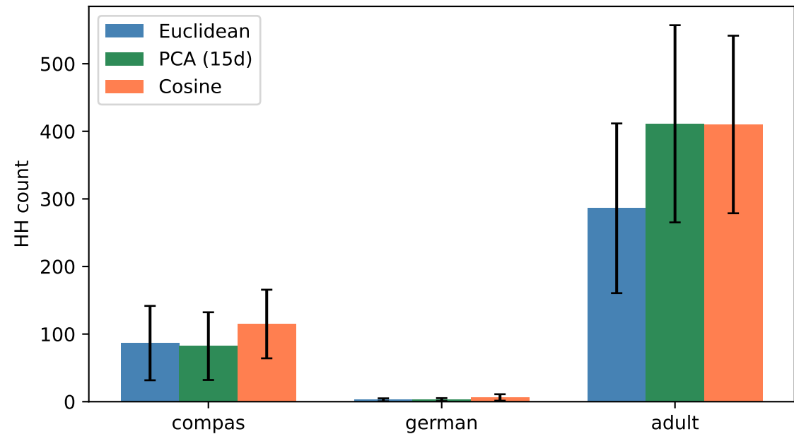
HH count
