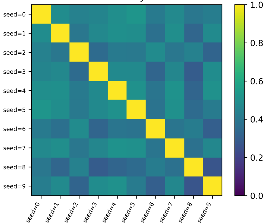
Variance-HH Jaccard
