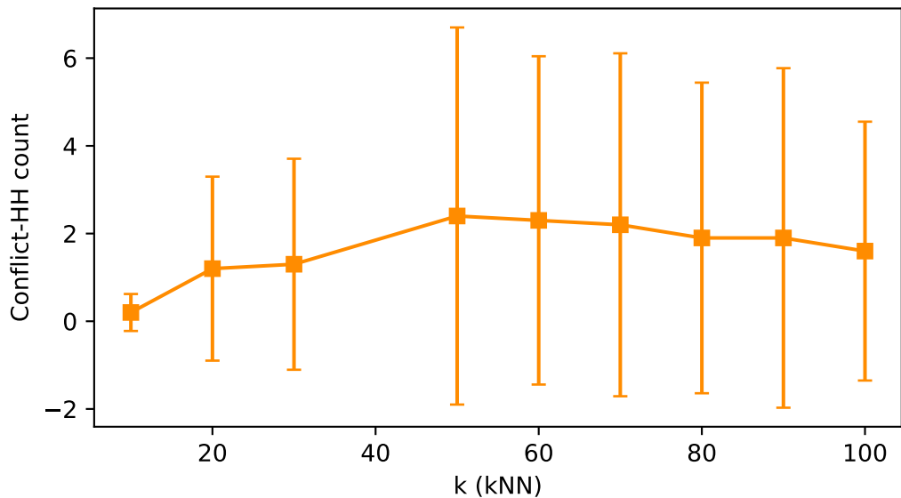
Conflict-HH count vs k
