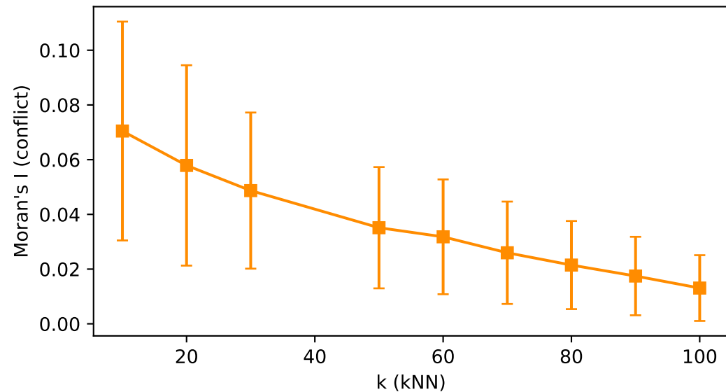
Moran's I (conflict) vs k
