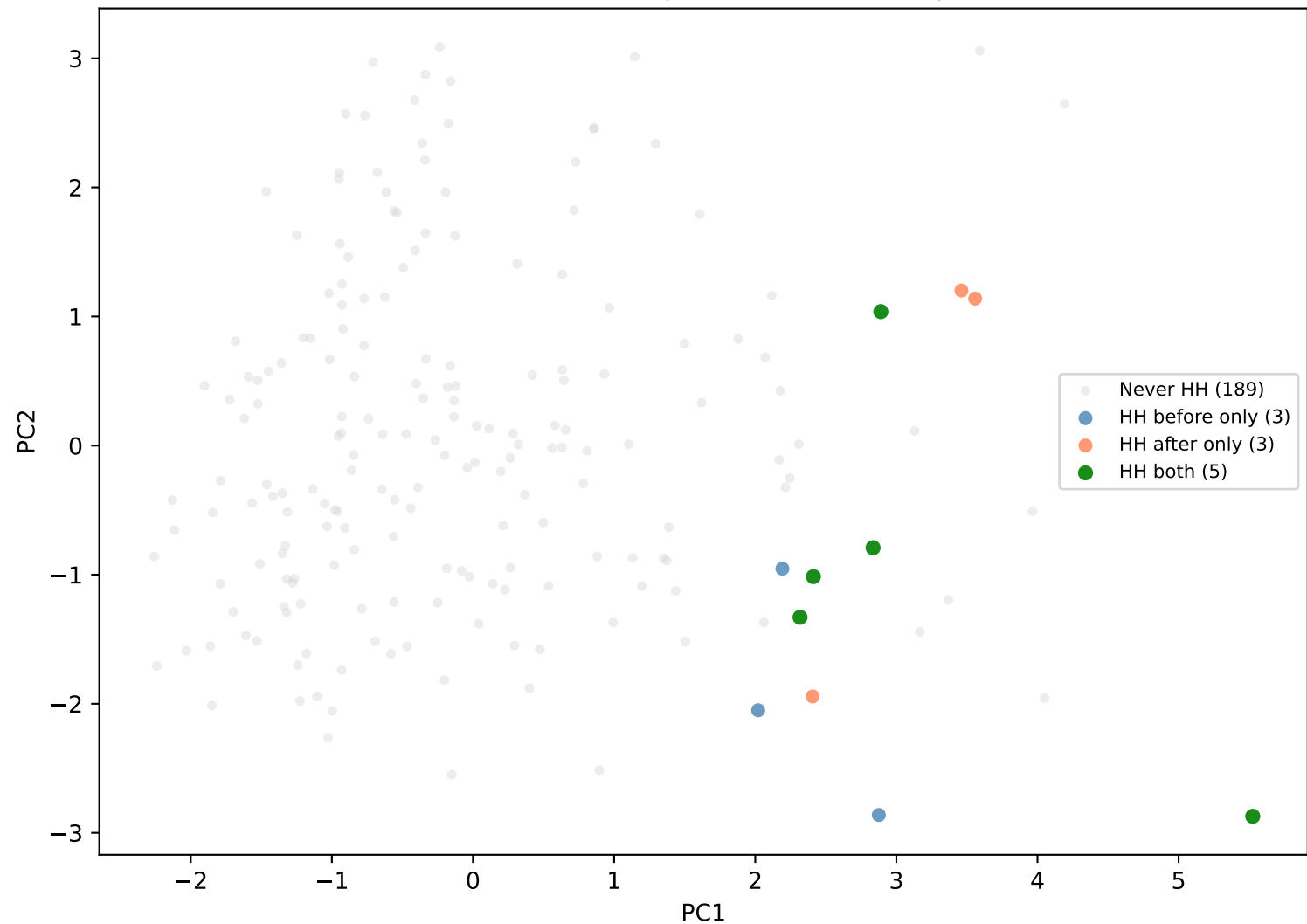
HH movement: before vs after platt calibration — german (seed=0)
