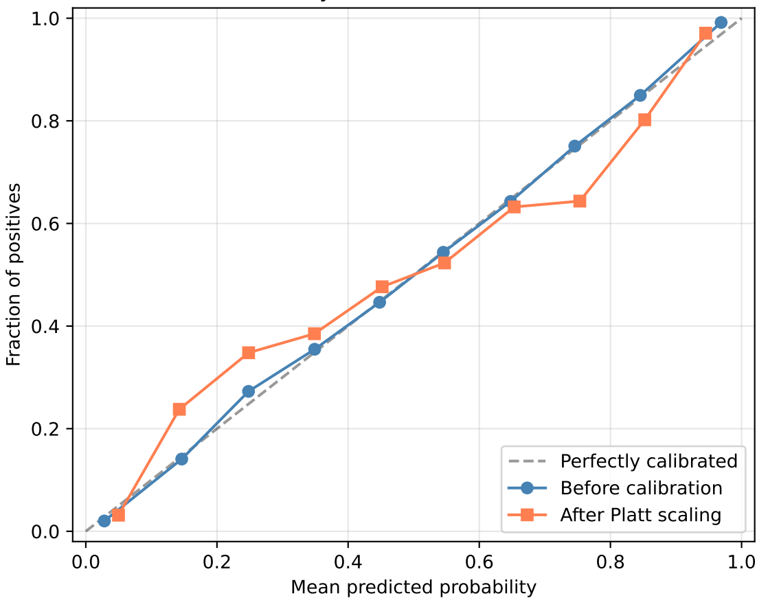
Reliability curve — adult (seed=4)
