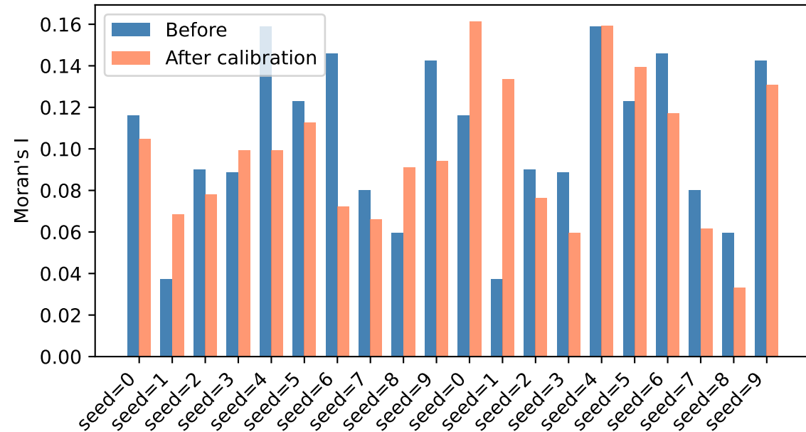
Moran's I: before vs after — german
