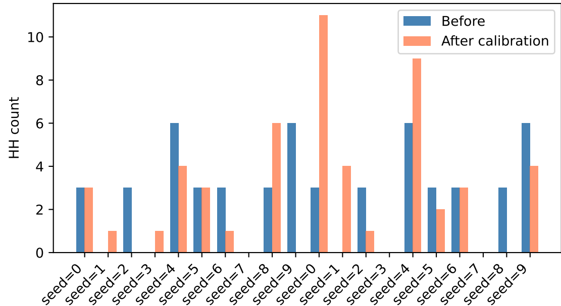
HH count: before vs after — german
