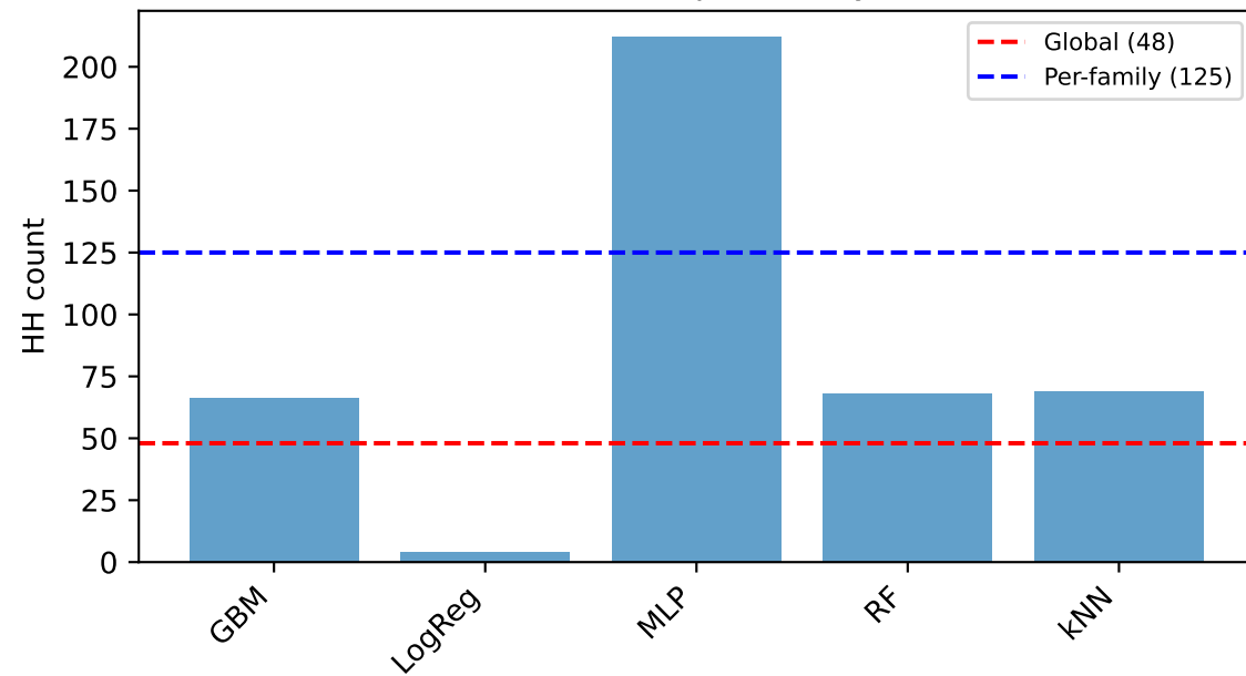
HH count per family
