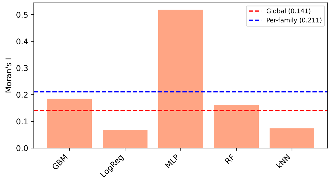
Moran's I per family
