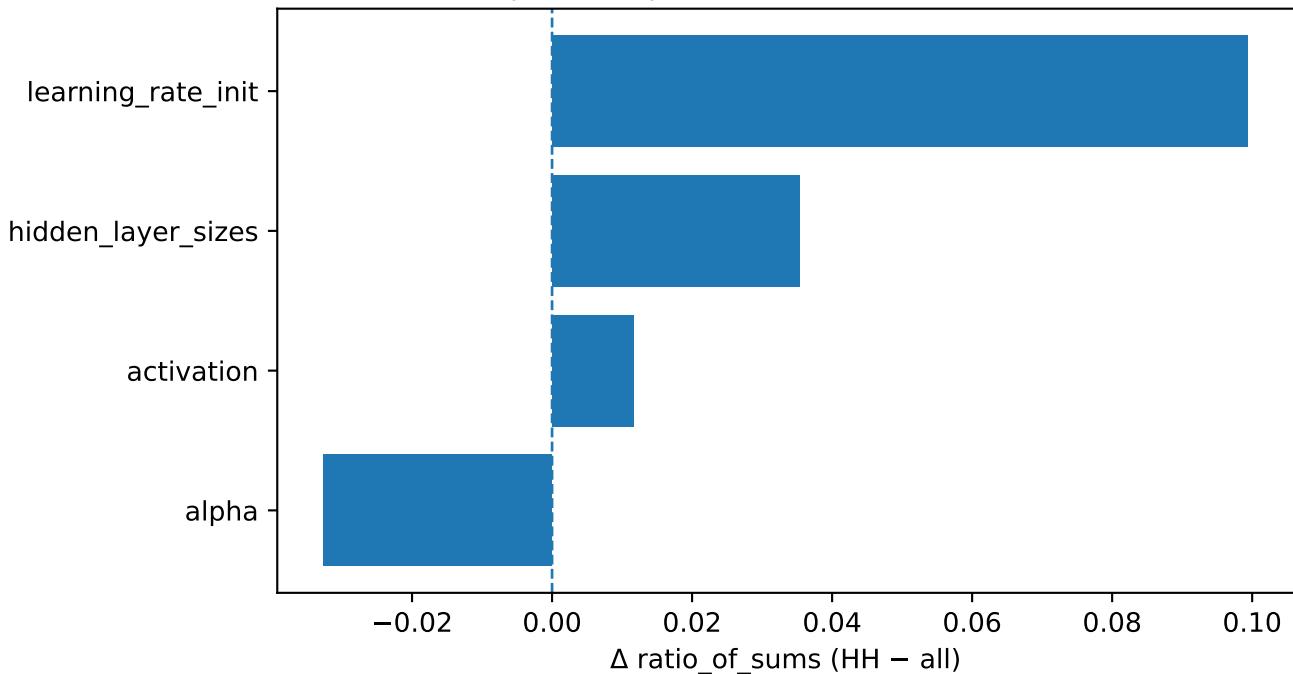
compas | seed 0 | MLP — HP importance shift in HH
