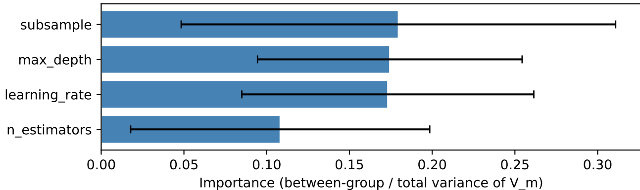
breast_cancer — GBM: top HP importance (mean \pm std over seeds)
