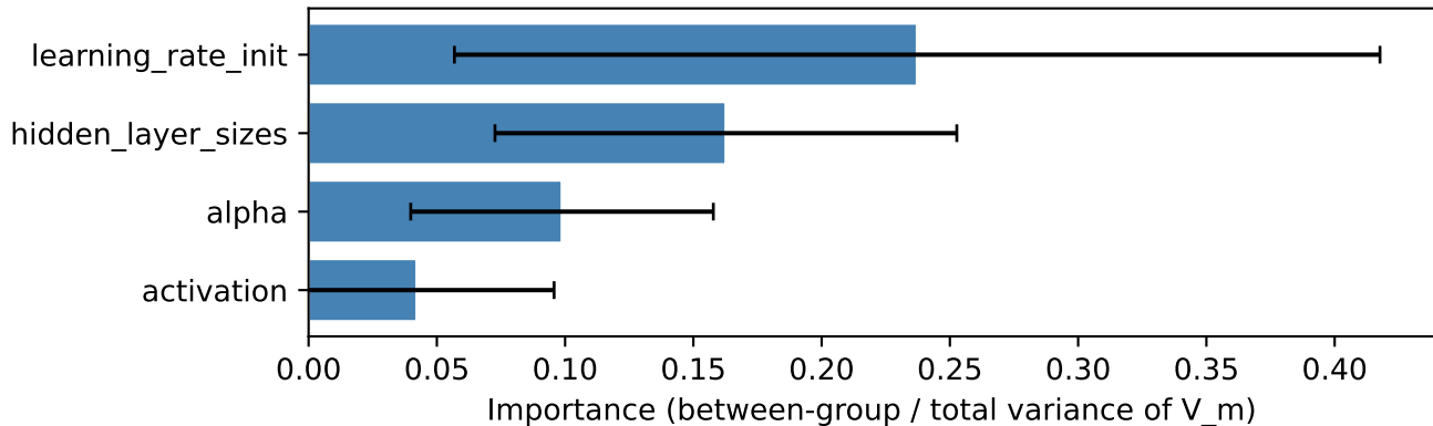
german — MLP: top HP importance (mean \pm std over seeds)
