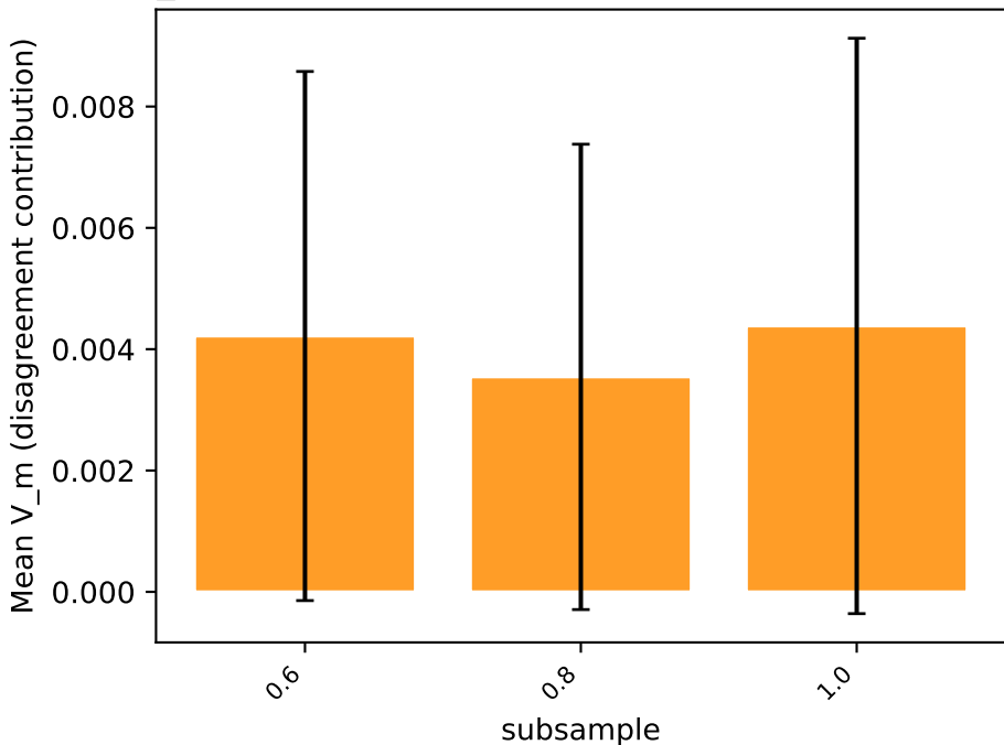
breast_cancer — GBM: marginal effect of subsample on V_m
