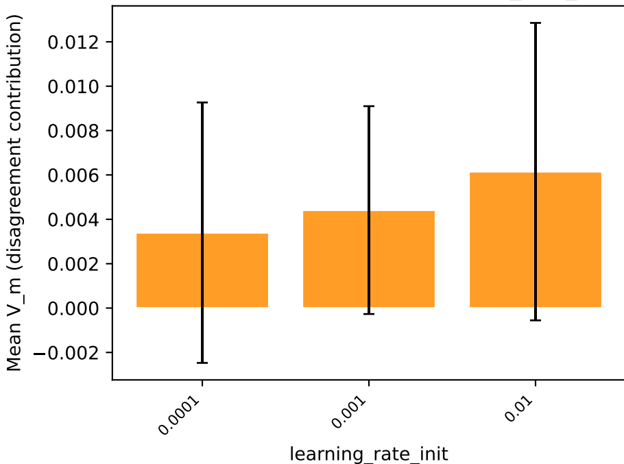
compas — MLP: marginal effect of learning_rate_init on V_m
