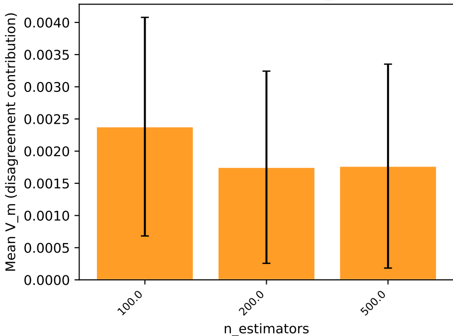
german — RF: marginal effect of n_estimators on V_m
