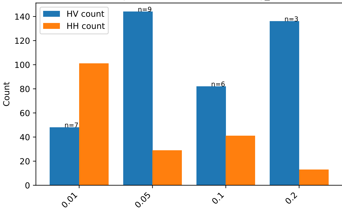
HP range effects: GBM " learning_rate
