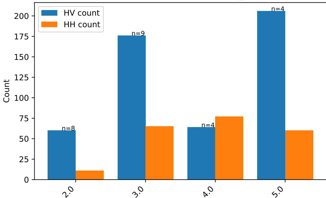
HP range effects: GBM " max_depth
