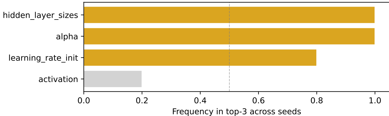
breast_cancer — MLP: rank stability (top-3 frequency)
