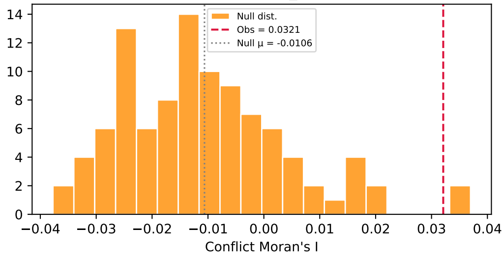
Conflict Moran's I (p_emp=0.030)
