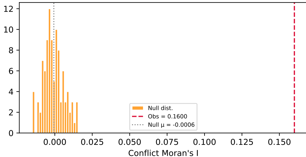
Conflict Moran's I (p_emp=0.010)
