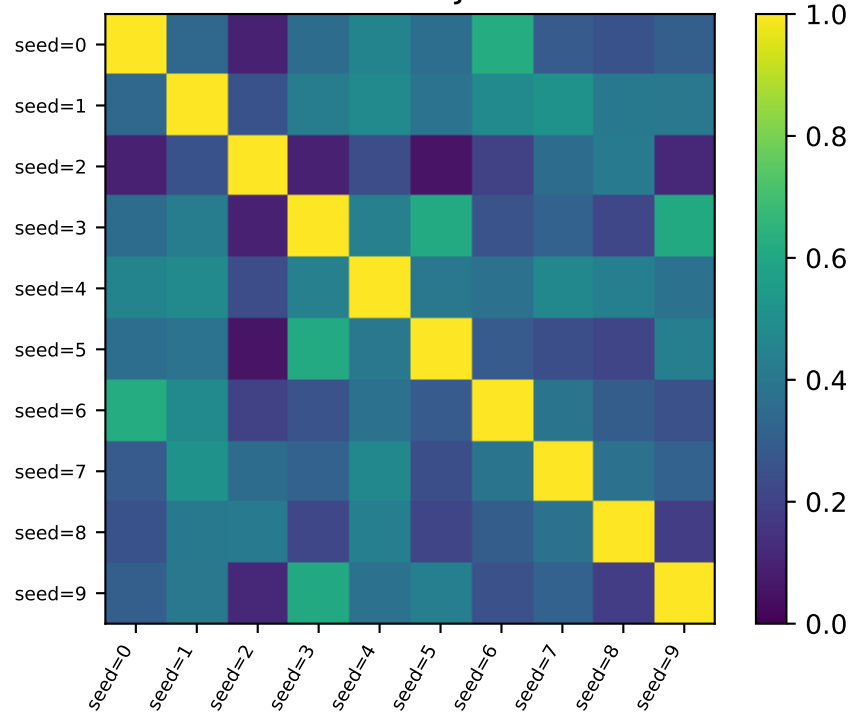
Variance-HH Jaccard
