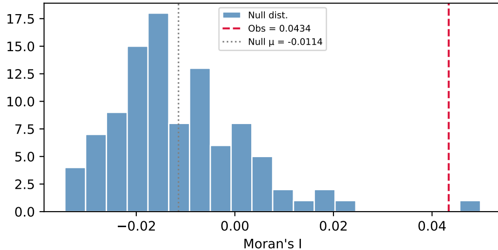
Moran's I (p_emp=0.020, p_pysal=0.008)
