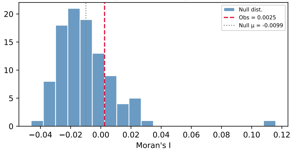
Moran's I (p_emp=0.208, p_pysal=0.168)
