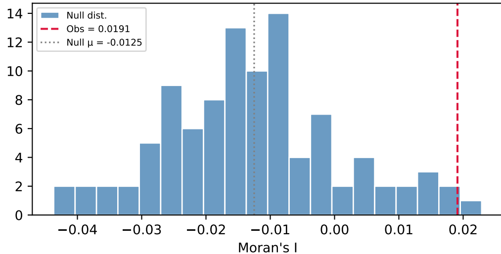
Moran's I (p_emp=0.020, p_pysal=0.011)
