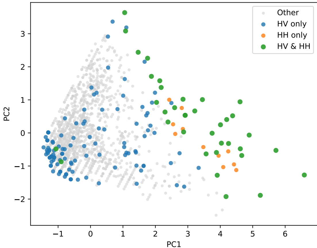
PCA: high-variance and HH regions (compas)
