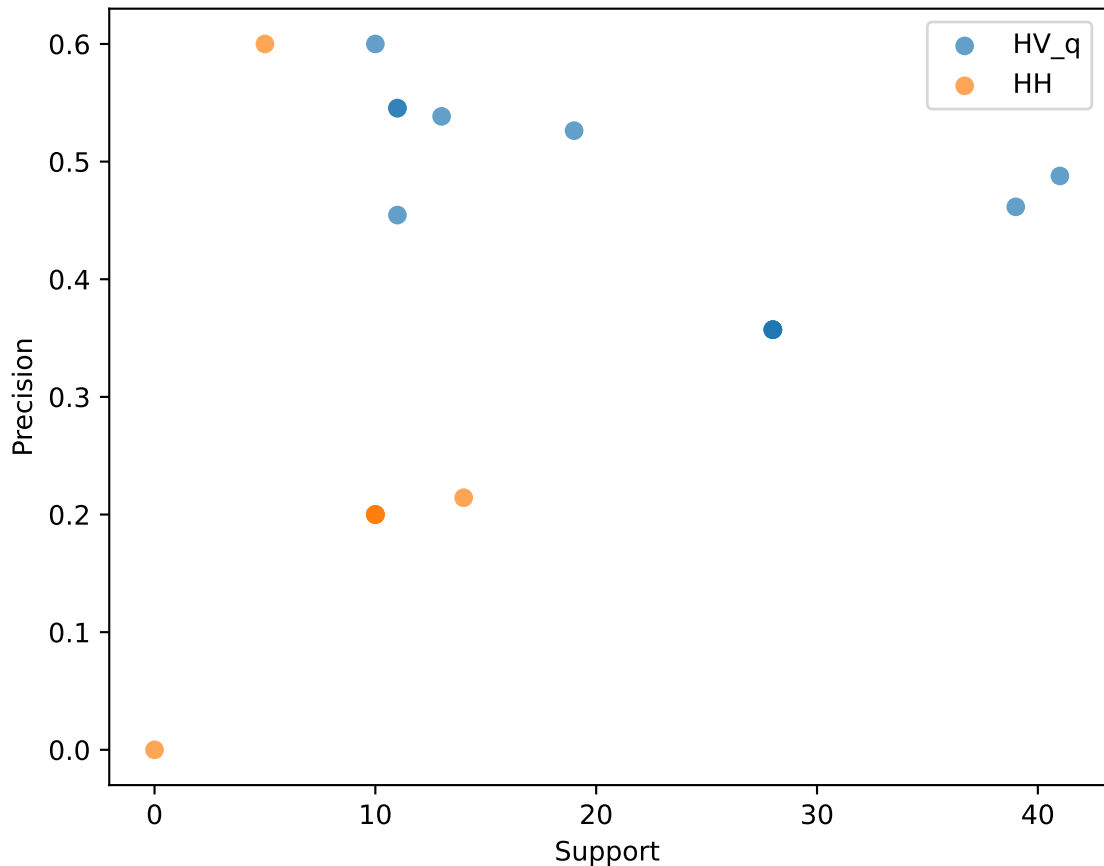
Rule tradeoff: support vs precision (german)
