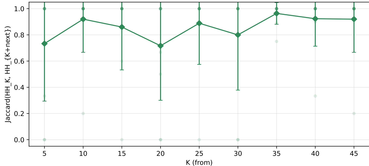
HH Jaccard between consecutive K — breast_cancer
