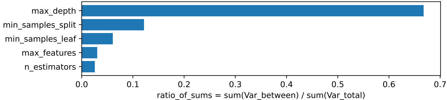
compas | seed=0 — RF: top hyperparameters (within-family)
