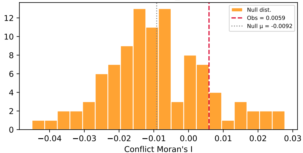
Conflict Moran's I (p_emp=0.149)
