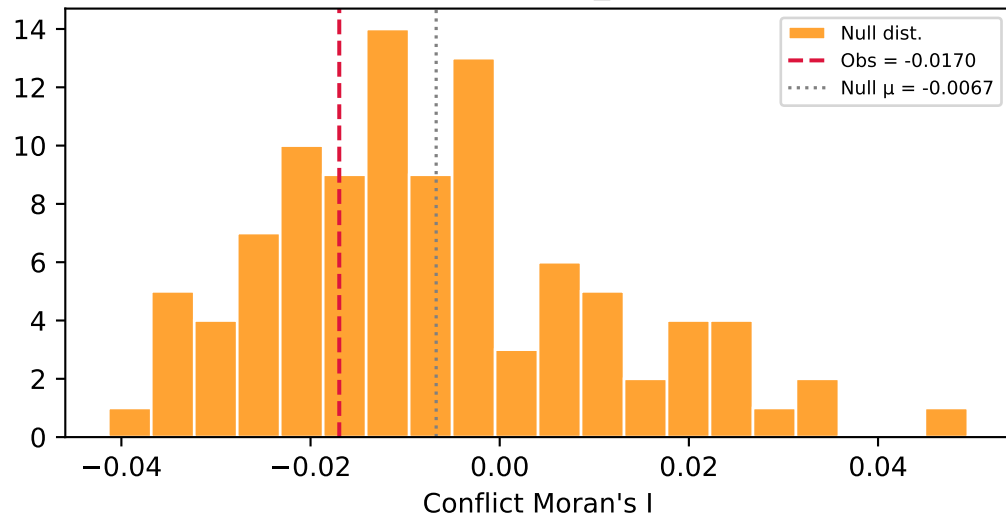
Conflict Moran's I (p_emp=0.713)
