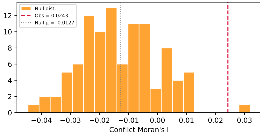
Conflict Moran's I (p_emp=0.020)
