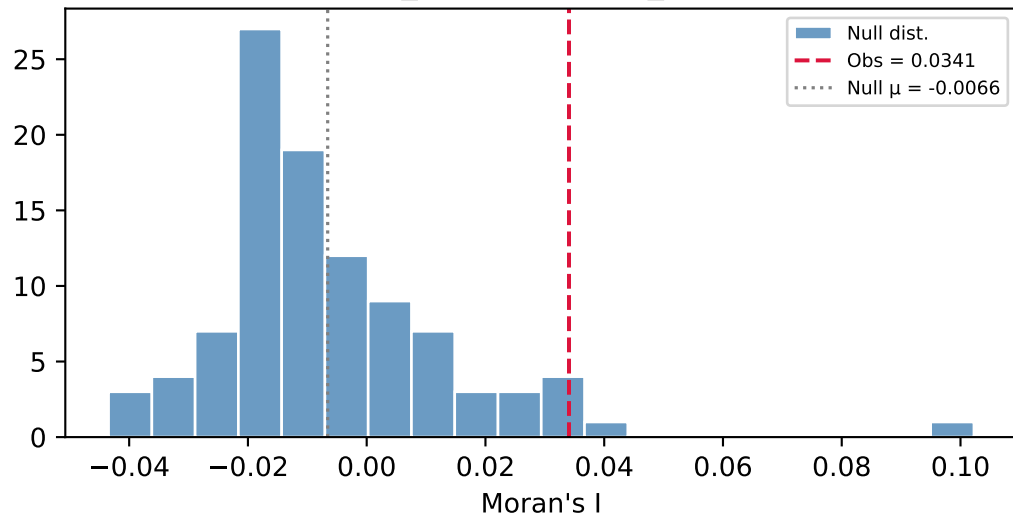
Moran's I (p_emp=0.030, p_pysal=0.020)
