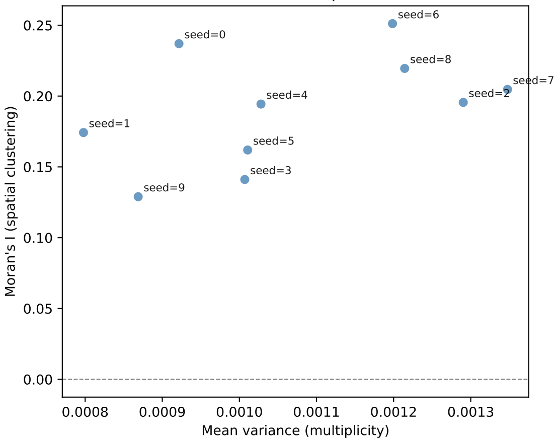
Mean variance vs Moran's I per run ( r = 0.477 )
