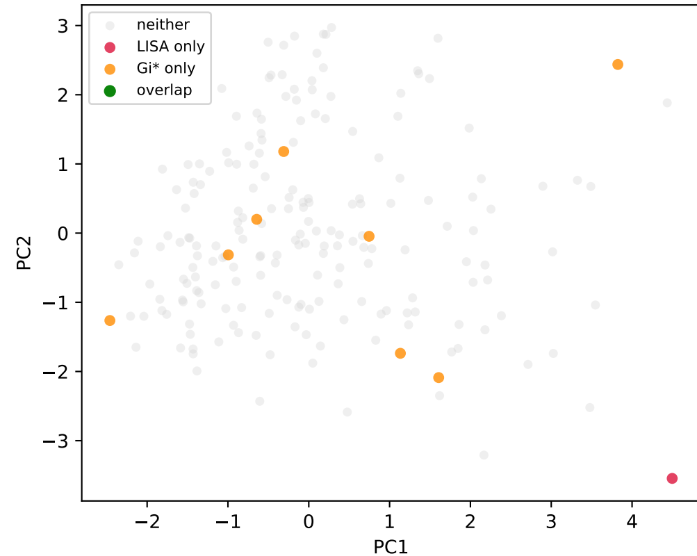
Overlap (Jaccard = 0.000)
